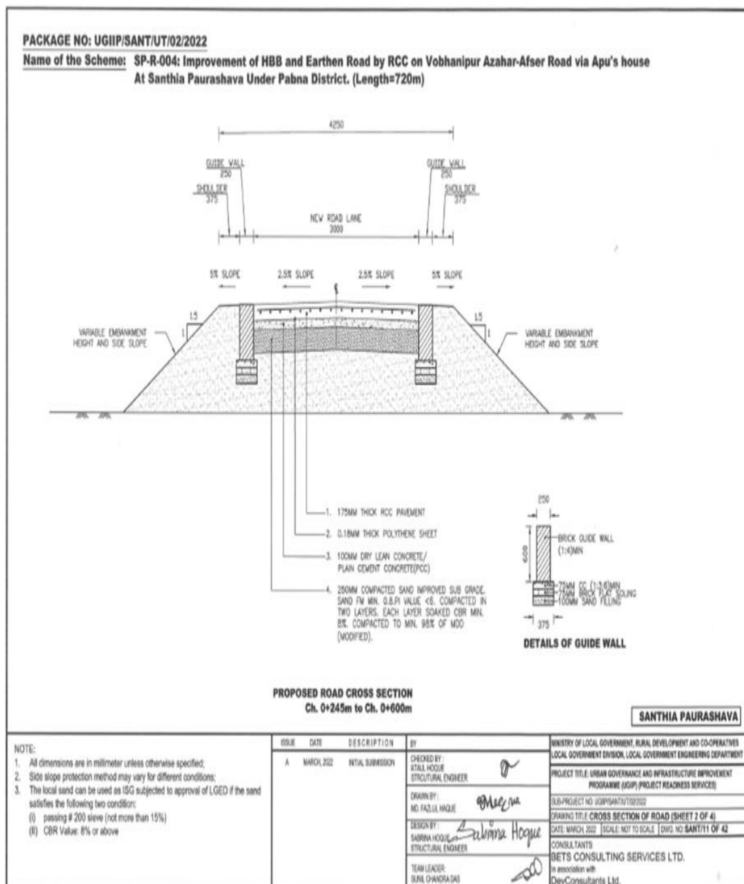
Figure 5: Cross-Section of Road in Pourashava
