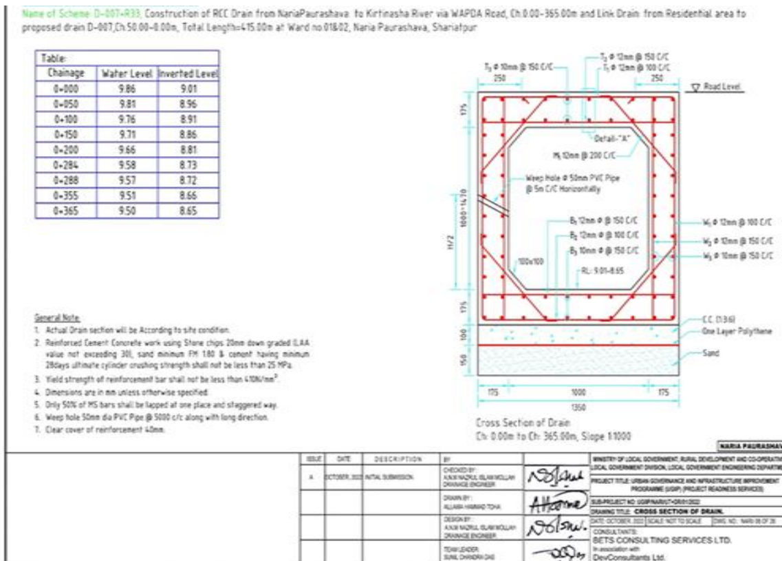
Figure 4: Cross-Section of Drain in Pourashava
