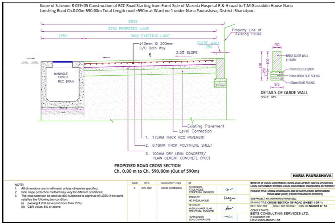
Figure 3: Cross-Section of Road in Pourashava
