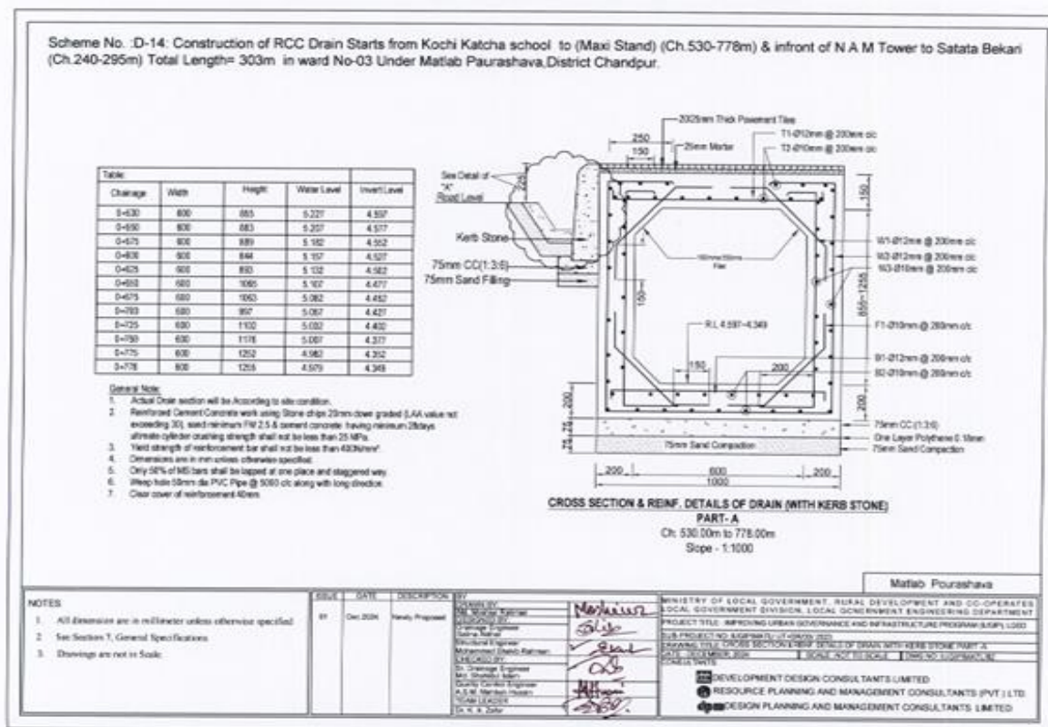
Figure 4: Cross-Section of Drain in Pourashava
