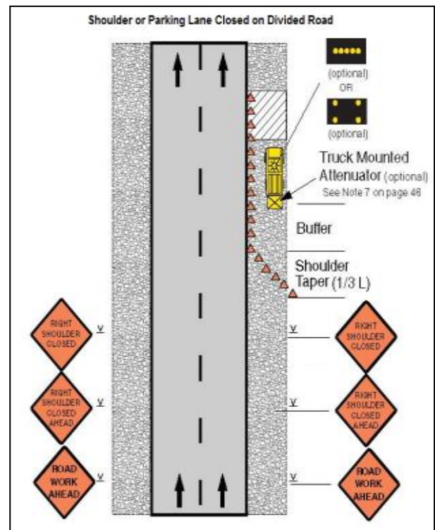
Figure A2 & A3: Work on shoulder or parking lane and shoulder or parking lane closed on divided road
