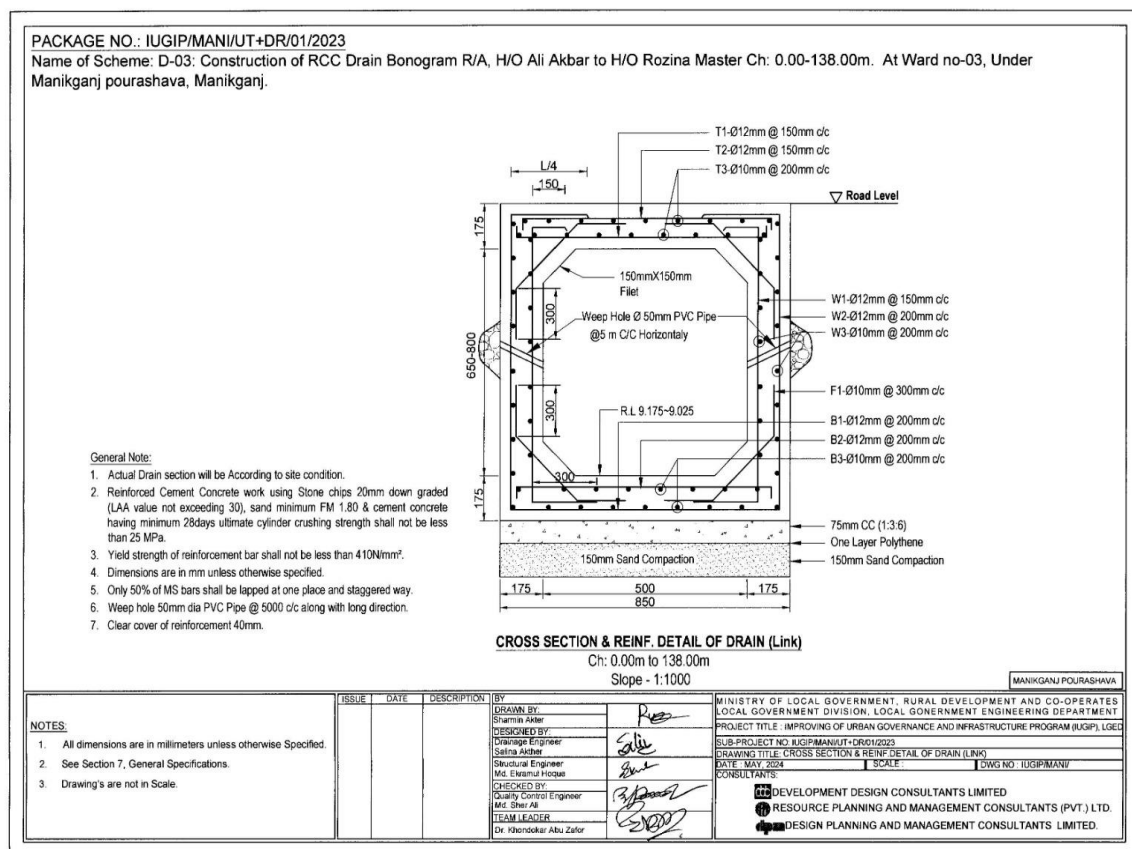
Figure 4: Cross-Section of Drain in Pourashava
