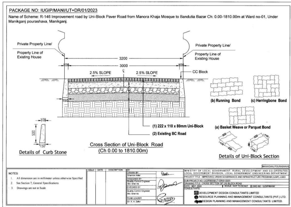
Figure 3: Cross-Section of Road in Pourashava
