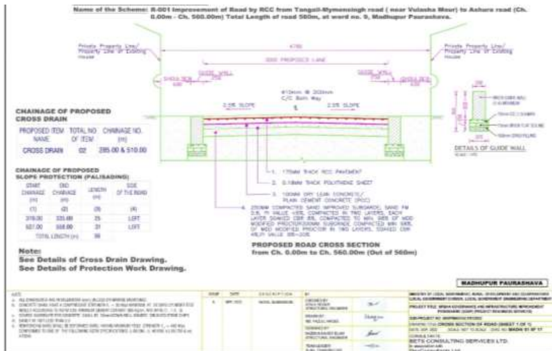
Figure 6: Cross-Section of Road in Pourashava
