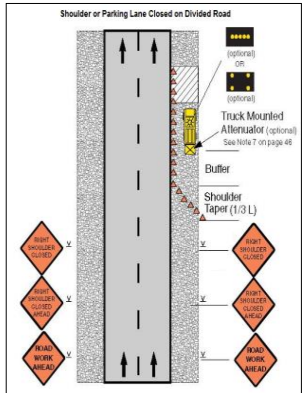
Figure A2 & A3: Work on shoulder or parking lane and shoulder or parking lane closed on divided road
