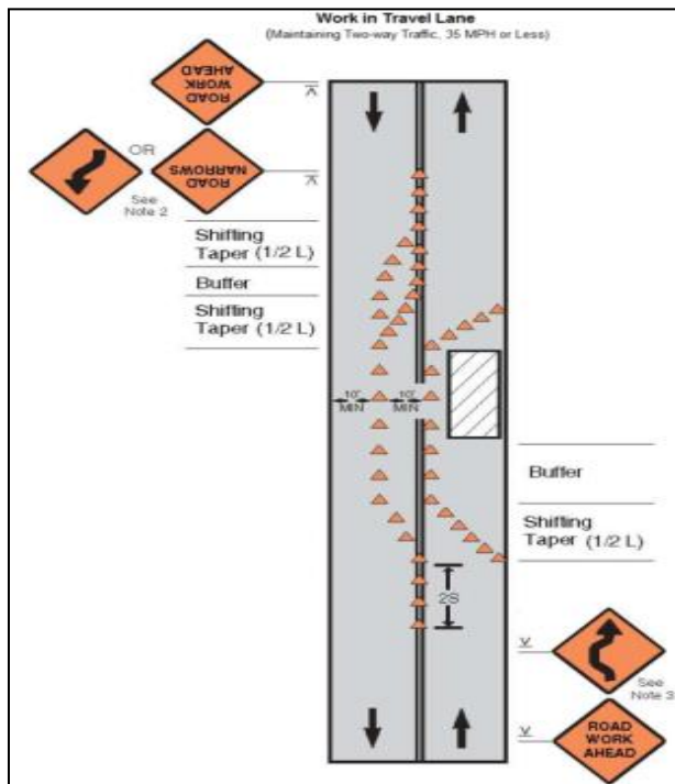
Figure A4 & A5: Work in Travel lane & Lane closure on road with low volume
