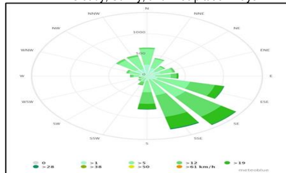
Wind Rose
