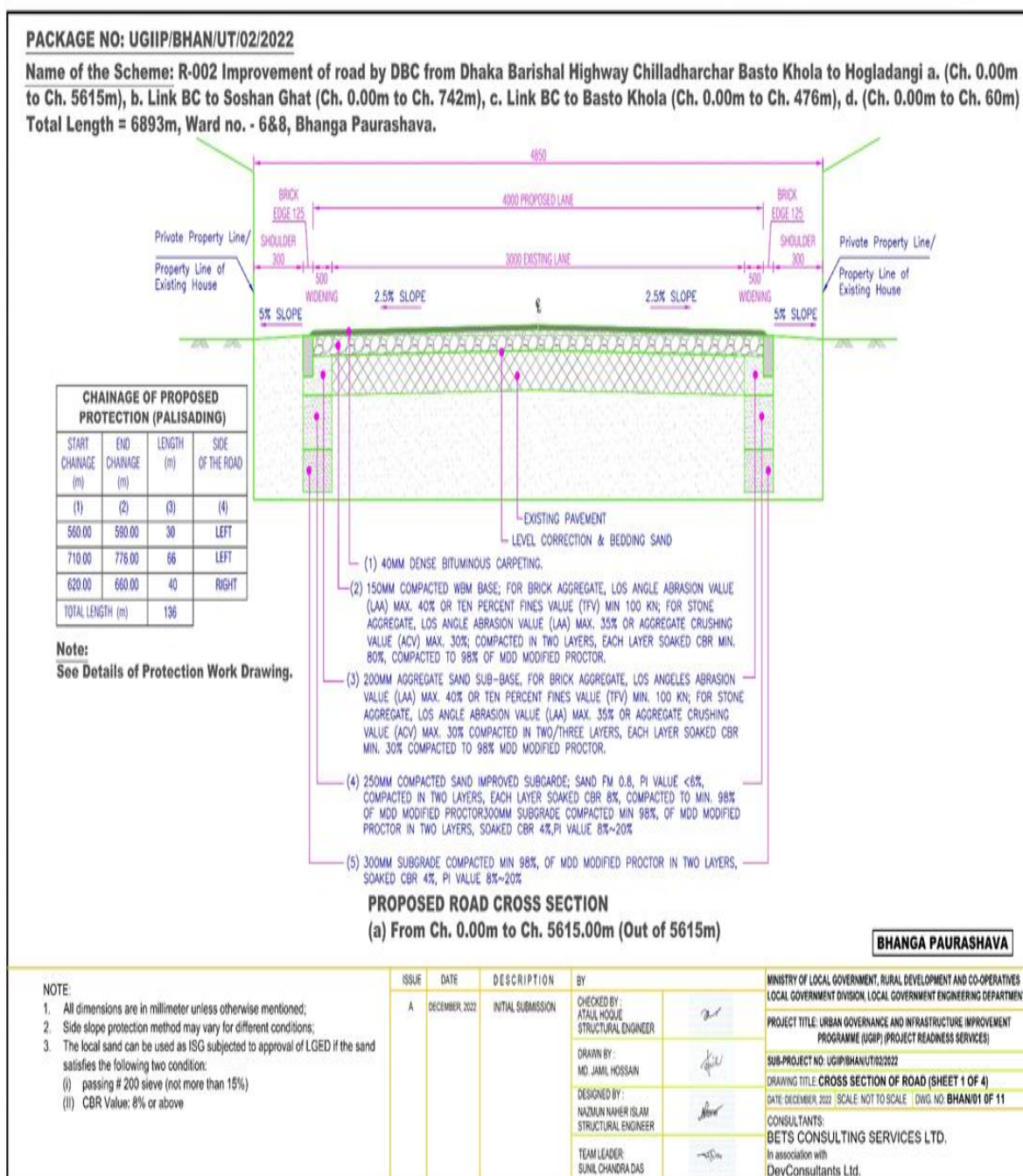
Figure 5: Cross-Section of Road in Bhanga Pourashava
