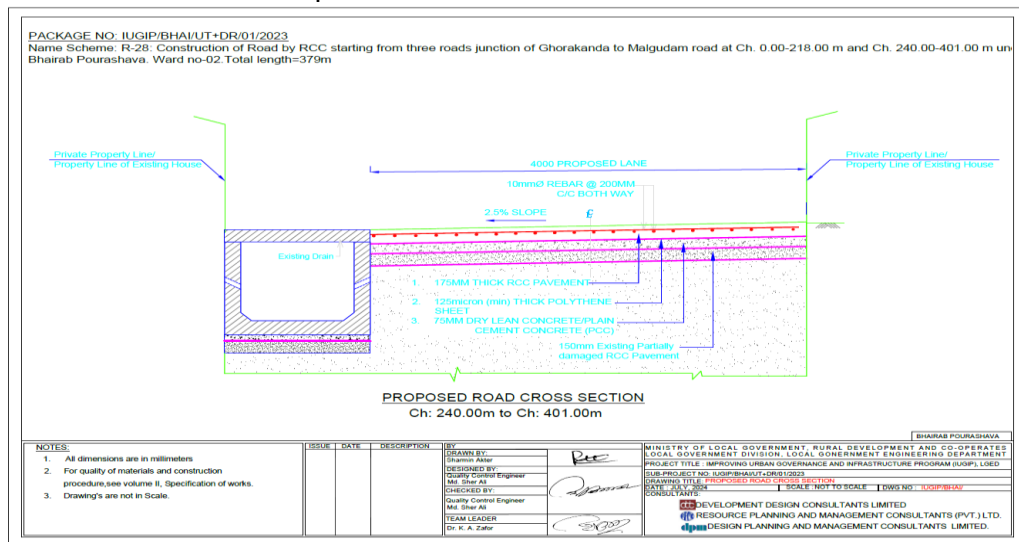
Figure III-3: Cross Section of Road in Bhairab Pourashava
