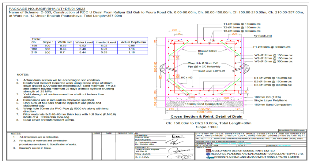
Figure III-4: Cross Section of Drain in Bhairab Pourashava
