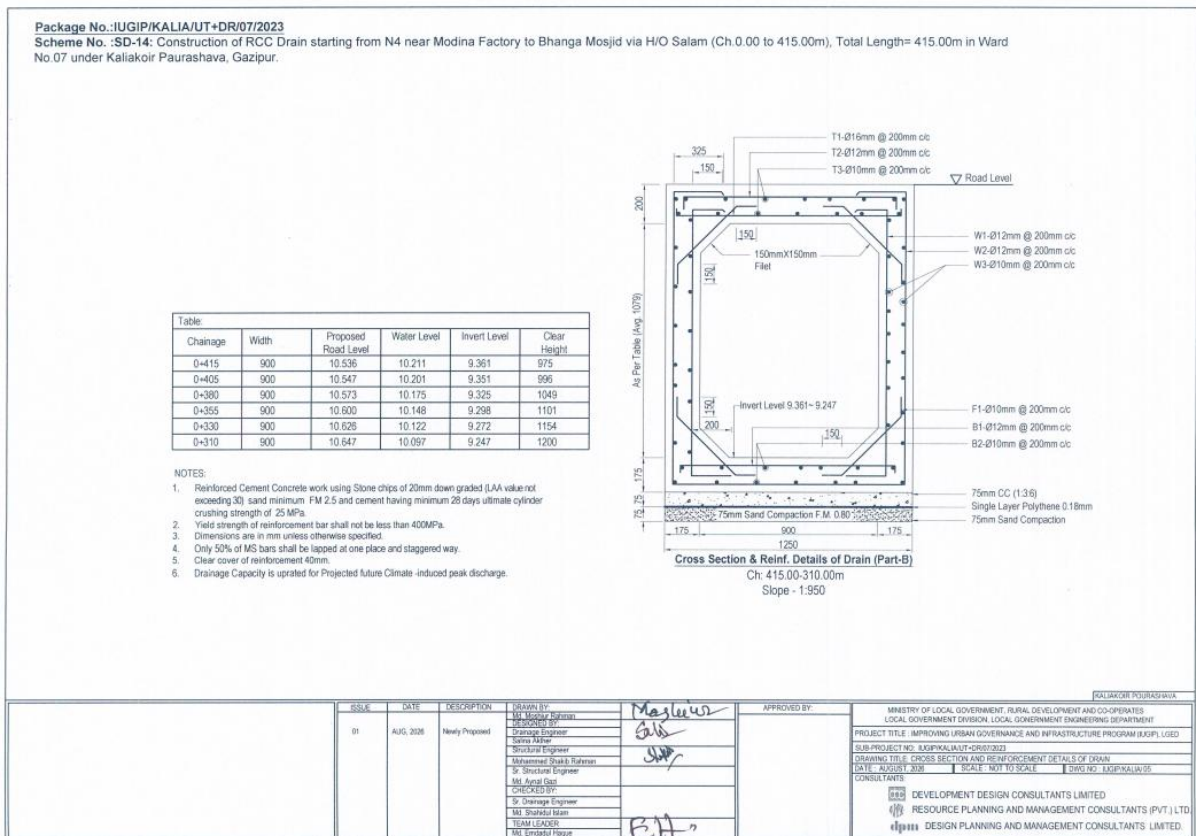
Figure 5: Cross-Section of Drain in Kaliakoir Pourashava
