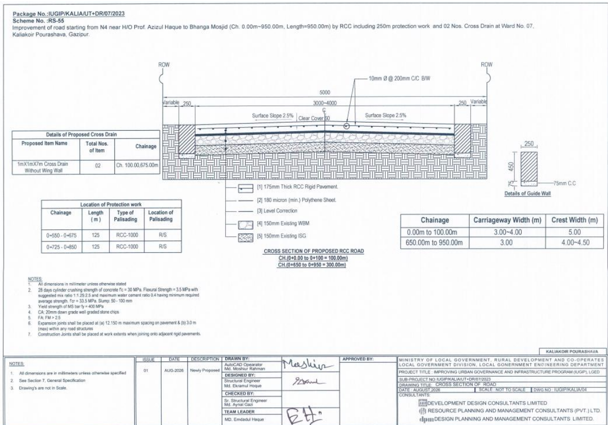
Figure 4: Cross-Section of Road in Kaliakoir Pourashava
