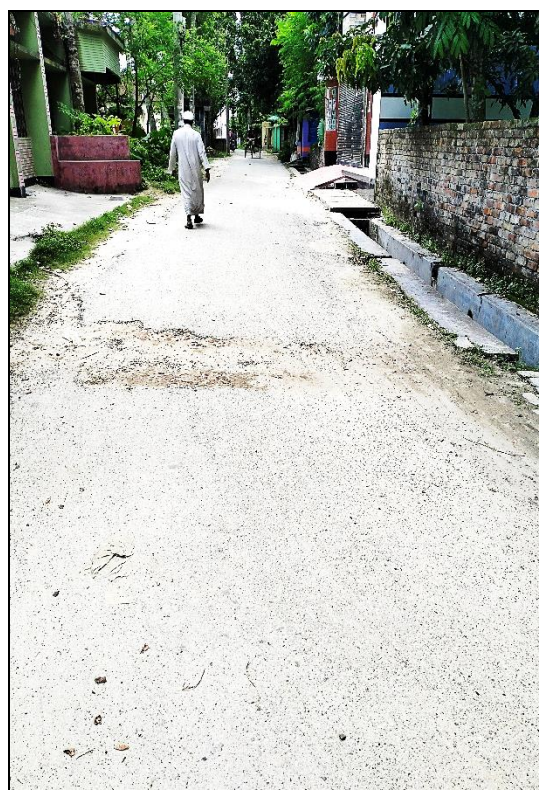
BHER-R-18: Improvement of road by Dense Bituminous Carpeting at Sayed Ali road a. (Ch. 0.00 to 765m) b. Link-1 (Ch. 0.00m to 125m) & installation of Street Light 32 nos. at Ward no. - 9, Bheramara Paurashava, Kushtia. Total Length = 890m.
