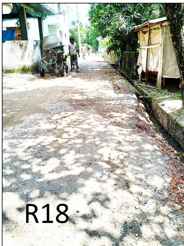
BHER-R-18: Improvement of road by Dense Bituminous Carpeting at Sayed Ali road a. (Ch. 0.00 to 765m) b. Link-1 (Ch. 0.00m to 125m) & installation of Street Light 32 nos. at Ward no. - 9, Bheramara Paurashava, Kushtia. Total Length = 890m.
